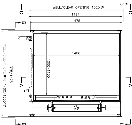
PLAN OF WELL 1:10
